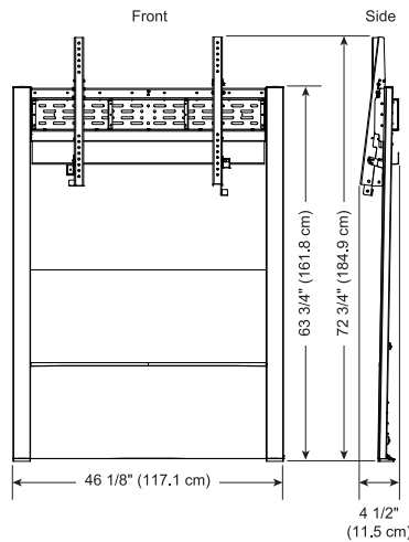
Wall stand with SMART Board 8084i-G4 interactive flat panel wall mount (WM-SBID-502)
