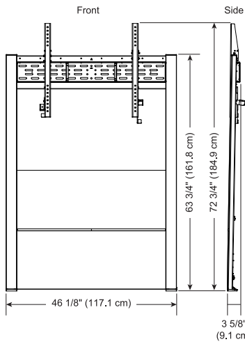
Wall stand with SMART Board 8070i-G4 interactive flat panel wall mount (WM-SBID-501)
